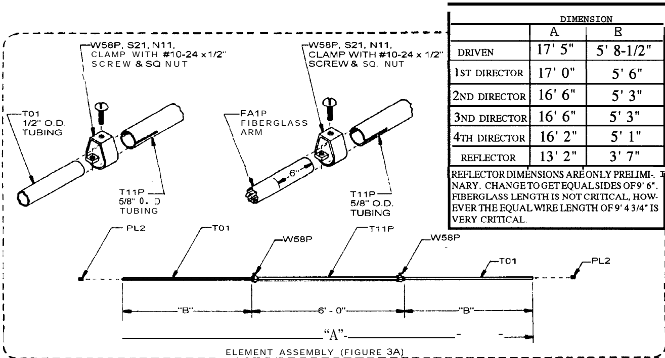
ELEMENT ASSEMBLY (FIGURE 3A)
